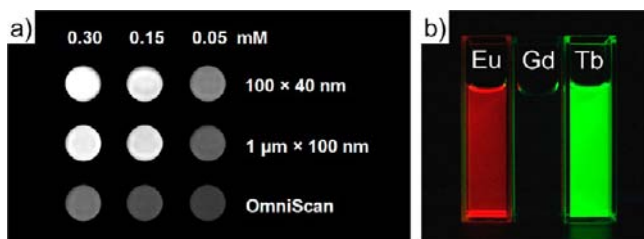
Figure 9. (a) T_1 -weighted MR phantom images of suspensions of \text{Gd}(\text{BDC})_{1.5}(\text{H}_2\text{O})_2 in water containing 0.1% xanthan gum as a dispersing agent. (b) Luminescence of ethanolic dispersions of Eu- and Tb-doped \text{Gd}(\text{BDC})_{1.5}(\text{H}_2\text{O})_2 when irradiated with UV light.
