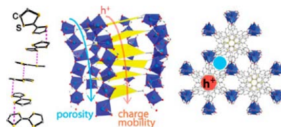
Figure 6. Left, electron transport pathway through a continuum of TTF moiety in the crystal structure of \text{Zn}_2(\text{TTFTB}) . Middle and right, crystal structure of \text{Zn}_2(\text{TTFTB}) showing porosity and charge transport through parallel channels. Reproduced with permission from ref 12d. Copyright, American Chemical Society 2012.
