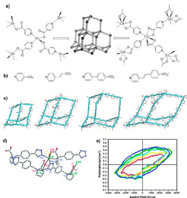
Figure 3. (a) Construction of MOFs with 3-D diamond structures from a linear pyridinecarboxylate ligand and Zn 2+ /Cd 2+ nodes. (b) Structures of linear pyridinecarboxylate ligands. (c) Diamondoid structures built from linear pyridinecarboxylate ligands. (d) Asymmetric unit of the crystal of Cd-TBP. (e) Electric field polarization cycles of Cd-TBP. (d) and (e) reproduced with permission from ref 39c. Copyright, American Chemical Society 2006.
