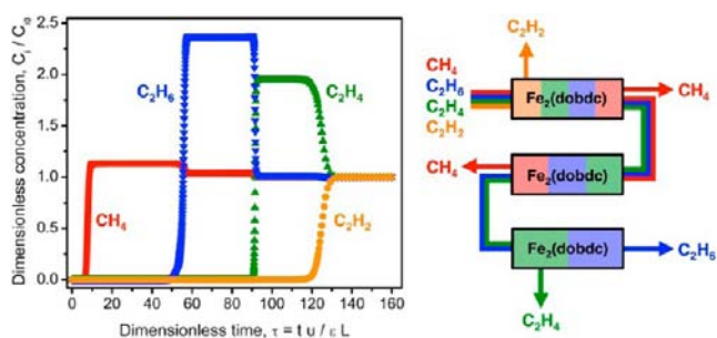
Figure 2. Left, calculated methane (red), ethane (blue), ethylene (green), and acetylene (orange) breakthrough curves for an equimolar mixture of the gases at 1 bar flowing through a fixed bed of Fe 2 (DOBDC) at 318 K. Right, schematic representation of the separation of a mixture of methane, ethane, ethylene, and acetylene using three packed beds of Fe 2 (DOBDC) in a vacuum swing adsorption or temperature swing adsorption process. Reproduced with permission from ref 34. Copyright, Science Magazine 2012.
