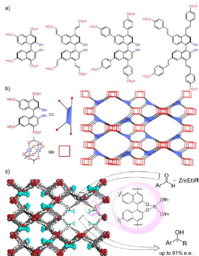
Figure 4. (a) Chemical structures of BINOL-derived tetracarboxylic acid ligands (BINOL-TC). (b) Representation of the BINOL-TC ligand as a blue distorted tetrahedron and the [\text{Cu}_2(\text{O}_2\text{CR})_4] paddlewheel as a red square, and simplified connectivity scheme of the MOF structure. (c) Schematic representation of asymmetric alkyl- and alkynylzinc additions catalyzed by the MOF-based Ti-BINOLate catalyst within large open channels. Reproduced with permission from ref 16f. Copyright, Nature Publishing Group 2010.
