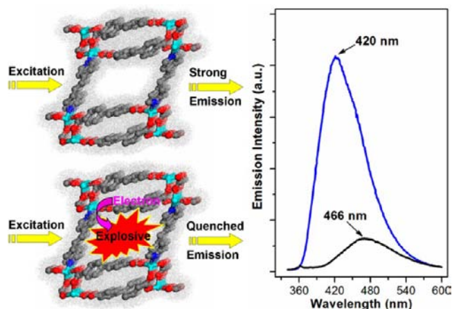
Figure 8. Luminescent quenching of [Zn_2(bpdc)_2(bpee)] by vapor of solid explosives DNT and DMNB for explosive detection. Reproduced with permission from ref 15b. Copyright, Wiley 2009.
