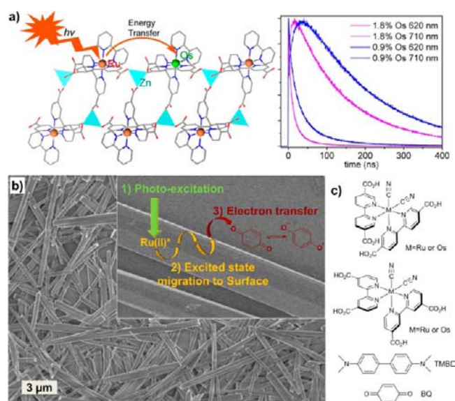
Figure 7. (a) Schematic showing energy transfer in a MOF crystal (left) and decay transients of \text{Ru}(\text{bipy})_3^{2+*} and \text{Os}(\text{bipy})_3^{2+*} in Os-doped MOFs built from \text{Ru}(\text{bipy})_3^{2+} derivatives (right). (b) Light-harvesting with a MOF microcrystal. The 3 MLCT excited states undergo rapid intraframework energy migration to carry out electron transfer quenching at the MOF/solution interface. (c) Chemical structures of the photoactive MOF building blocks and reductive tetramethylbenzidine (TMBD) and oxidative benzoquinone (BQ) quenchers. Reproduced with permission from refs 19a (a) and 19b (b and c). Copyright, American Chemical Society 2009 and 2010.
