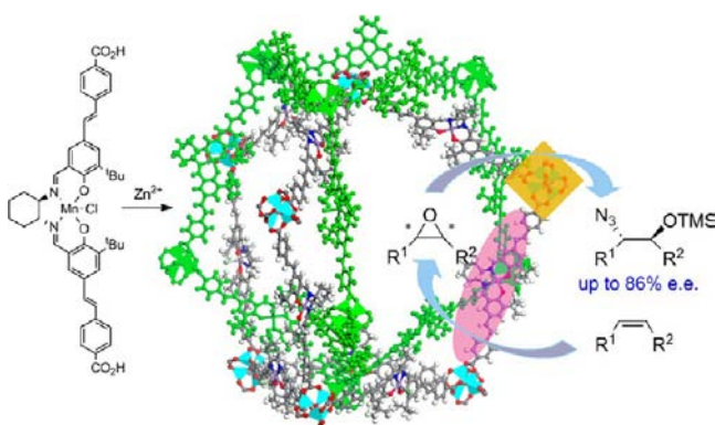
Figure 5. Schematic representation of sequential asymmetric epoxidation and ring-opening reactions catalyzed by the Mn-Salen-based ligand and [\text{Zn}_4(\mu_4\text{-O})(\text{CO}_2)_6] SBU, respectively. Reproduced with permission from ref 16g. Copyright, Royal Society of Chemistry 2011.
